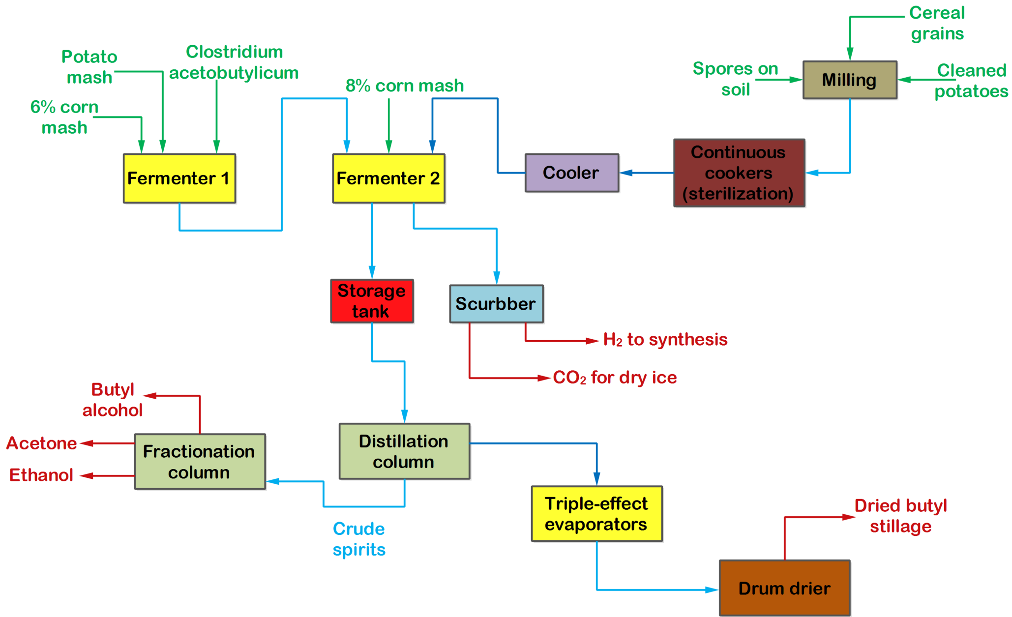
Figure: Manufacture of Butyl alcohol by fermentation of starch products
